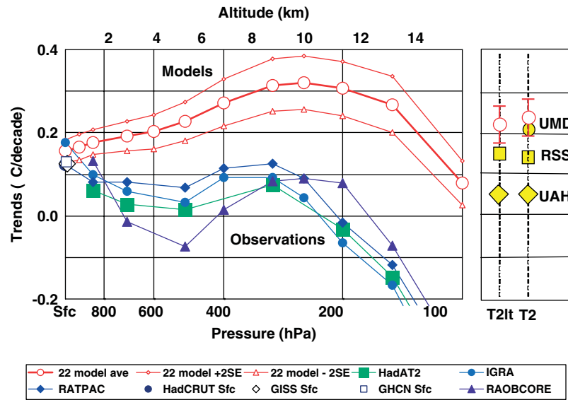
Figure 1. Temperature trends for the satellite era. Plot of temperature trend (C/decade) against pressure (altitude) from the data in Tables I and II. The HadCRUT2v surface trend value is a large blue circle. The GHCN and the GISS surface values are the open rectangle and diamond. The four radiosonde results (IGRA, RATPAC, HadAT2, and RAOBCORE) are shown in blue, light blue, green, and purple respectively. The two UAH MSU data points are shown as gold-filled diamonds and the RSS MSU data points as gold-filled squares. The MSU UMD data point is gold circle. The 22-model ensemble average is a solid red line. The 22-model average \pm 2\sigma_{SE} are shown as lighter red lines. Some of the values for the models for 1000 hPa are not consistent with the surface value or the value at 925 hPa. This is probably because some model values for p = 1000 hPa are unrealistic; they may be below the surface. So instead of using the values for p = 1000 hPa we used the surface values. MSU values of T_{2LT} and T_2 are shown in the panel to the right. UAH values are yellow-filled diamonds, RSS are yellow-filled squares, and UMD is a yellow-filled circle. Synthetic model values from Table III are shown as white-filled circles, with 2\sigma_{SE} uncertainty limits as error bars. From the text, the uncertainties of the observational datasets are: surface, \pm 0.04 C/decade; radiosondes, \pm 0.10 C/decade; MSU satellites, \pm 0.10 C/decade. At the surface, the mean of the models and the observations are seen to agree within the uncertainties; hence the overlap of symbols.
